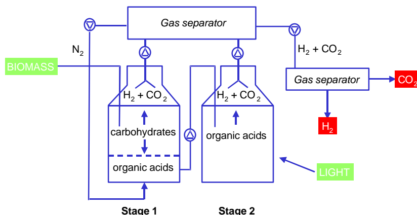
H 2 Production from biomass in a 2 stage fermentation
